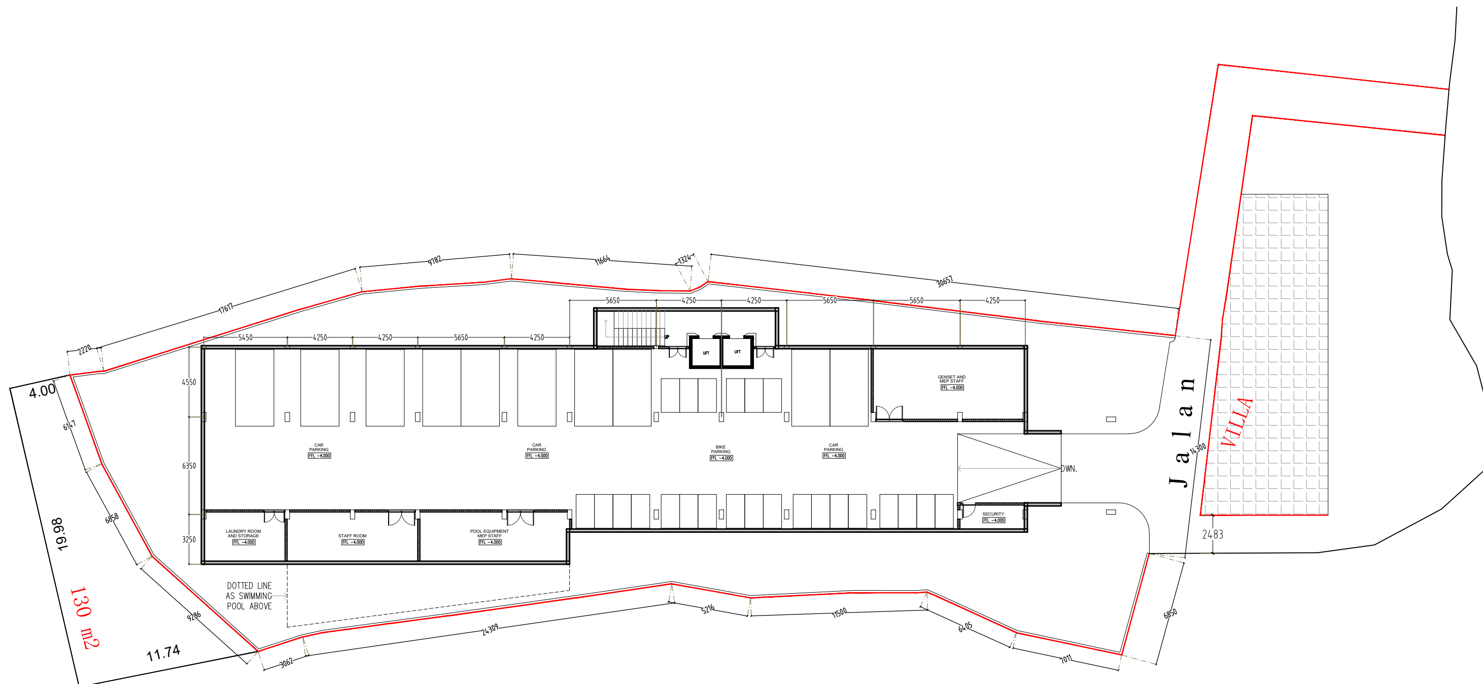
- BASEMENT FLOOR - 1 : 250 - A3
